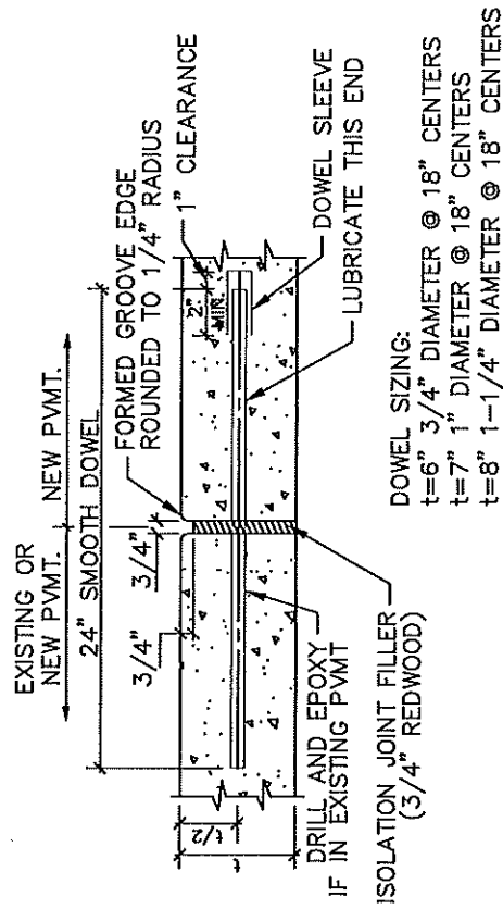
EXPANSION JOINT
