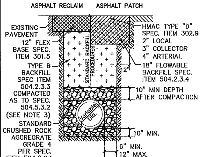
ASPHALT PAVEMENT
