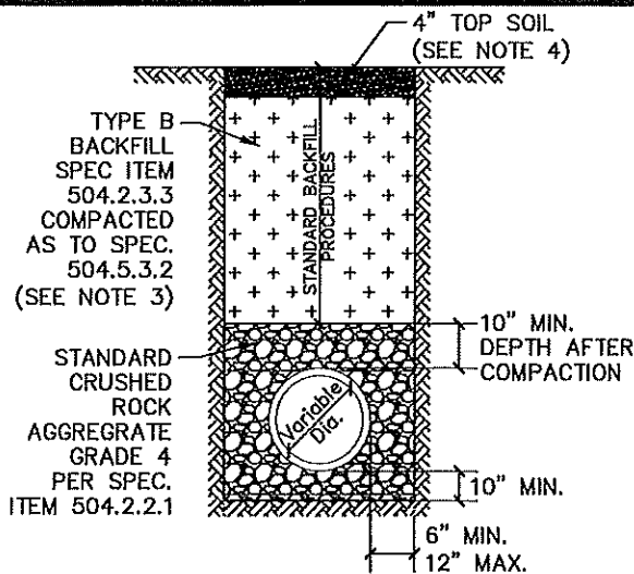
UNPAVED AREA
