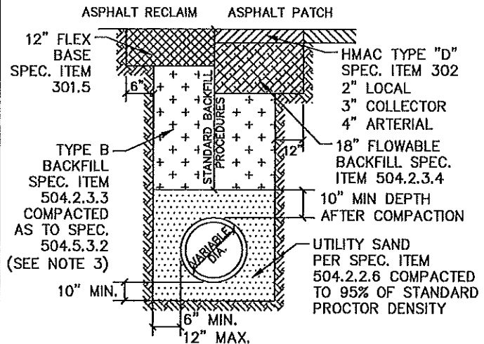
ASPHALT PAVEMENT
