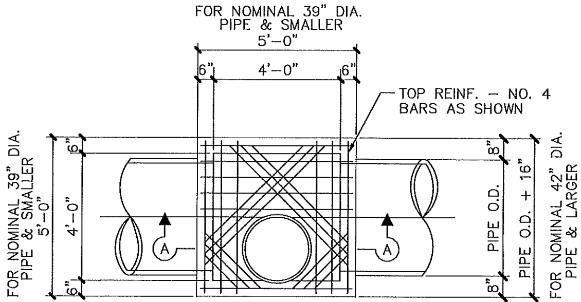
PLAN VIEW
