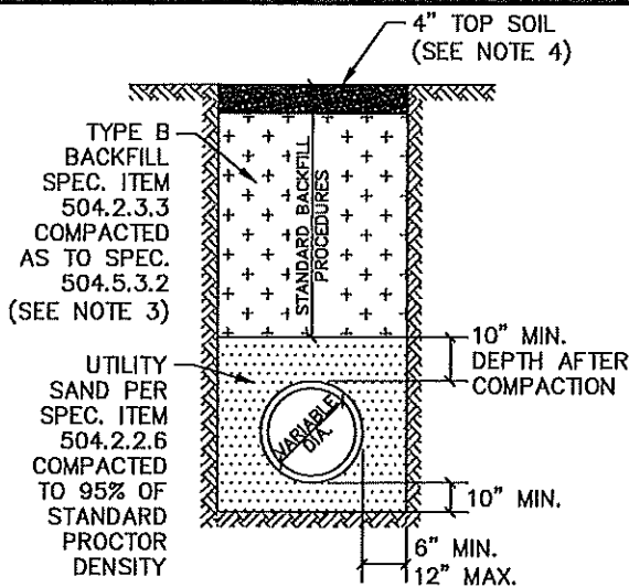
UNPAVED AREA
