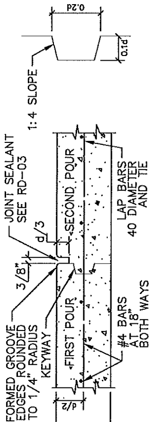
TRANSVERSE OR LONGITUDINAL CONSTRUCTION JOINT
