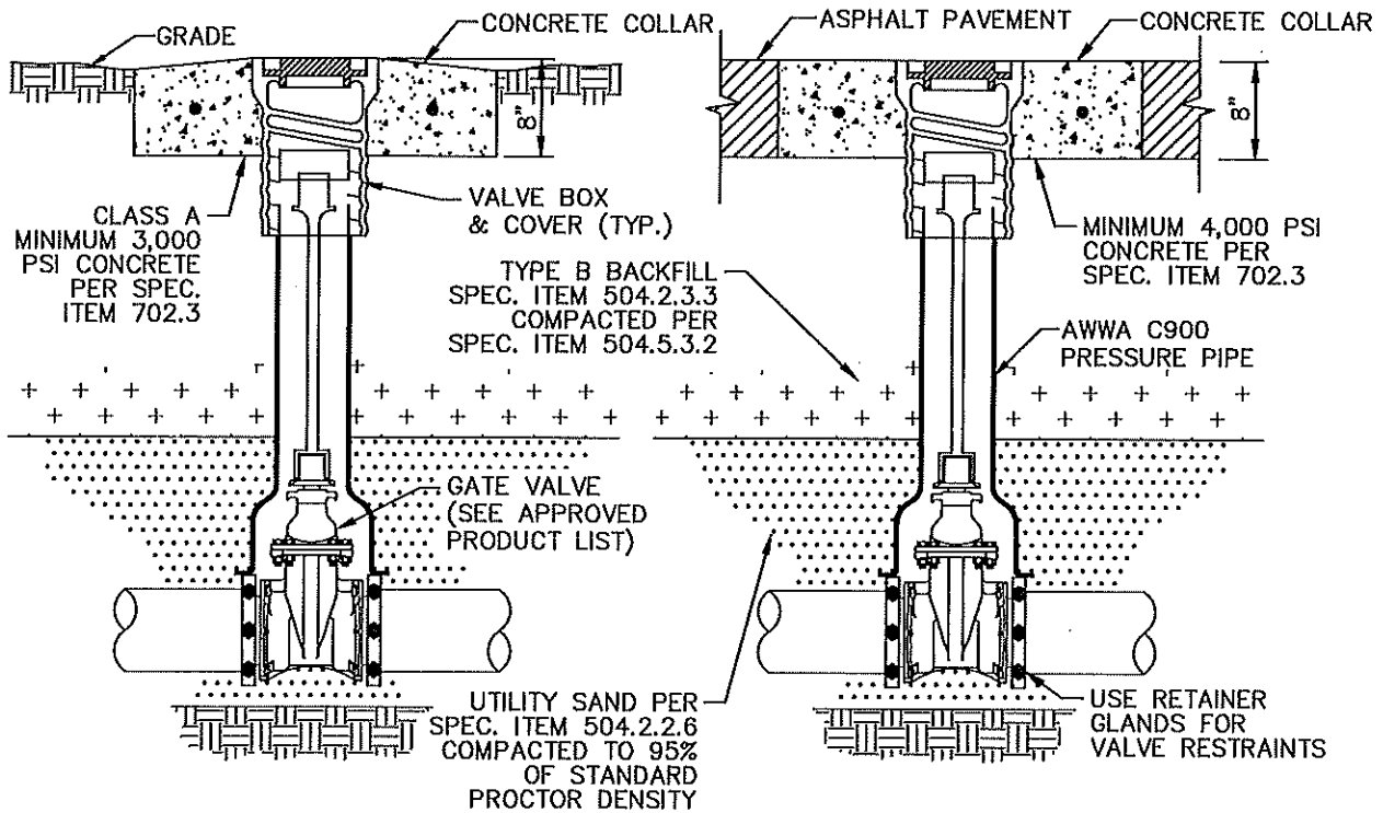
CONCRETE COLLAR
