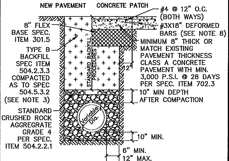
CONCRETE PAVEMENT
